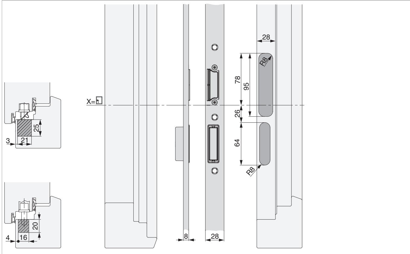
Detail B
